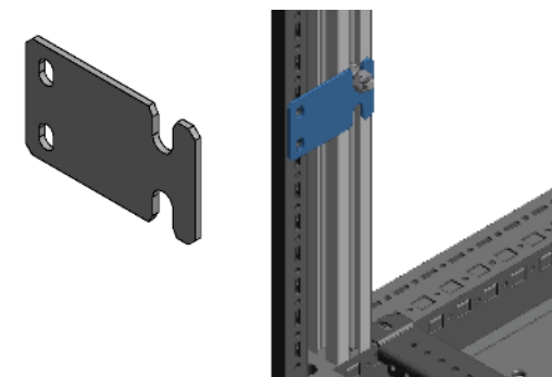
MBS.070 Adaptionss- platte TS8
